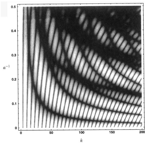
FIG. 2. A plot of S_a(k) . White corresponds to a value of 1, while dark corresponds to small values. The intensity is approximately linear in the logarithm of S_a(k) . Note the extreme values a = 2 and a = \infty for which there are explicit expressions for S_a(k) , given in Eqs. (17) and (18). The multiple zeros occurring at odd integral a are clearly visible.
